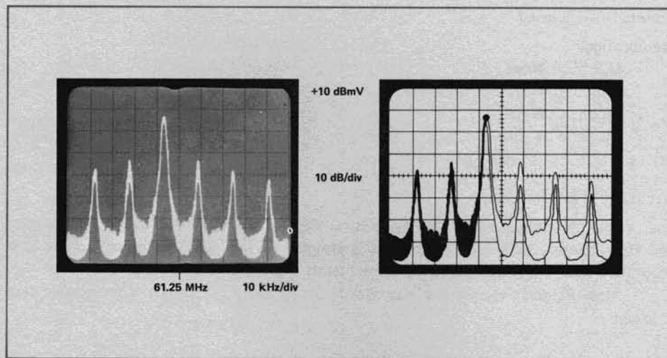
Figure 4.2 Using Tracking Generator, Manually Scan to Peak of Signal
