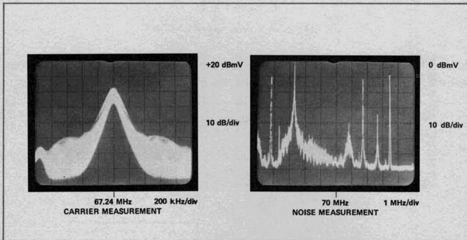
Figure 3.2 Carrier level is + 2 dBmV, and noise level is - 66 dBmV at 70 MHz. C/N Ratio (after correction) is 40 dB in 4 MHz.
