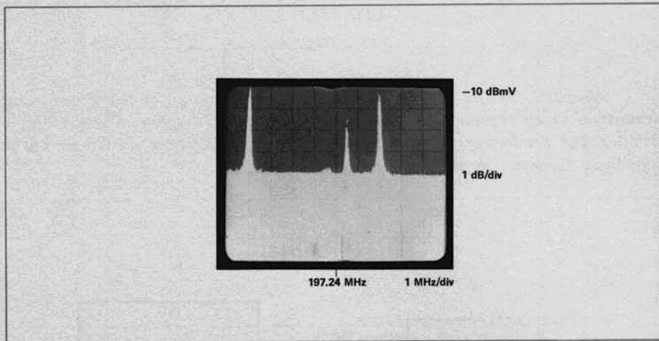
Figure 9.2 Flatness Sweep of a Single Channel
