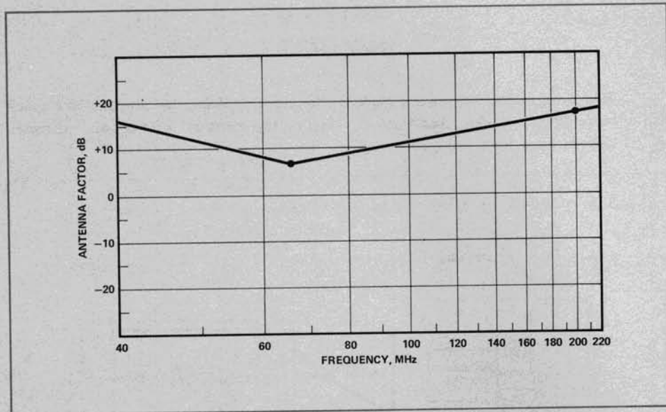
Figure 8.2 Antenna Factor, Singer MD-105-T1
