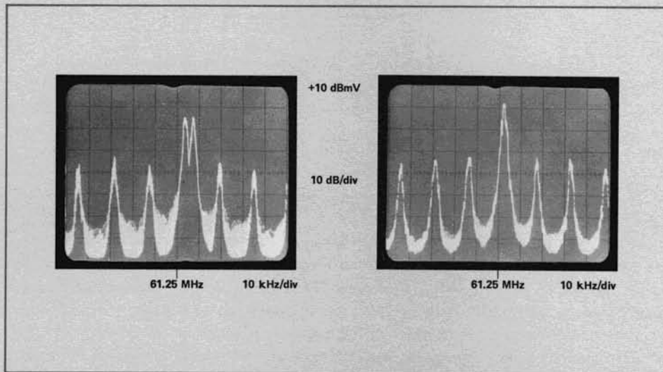
Figure 4.3 Superimpose Substitution Oscillator, and Read Frequency on Counter.
