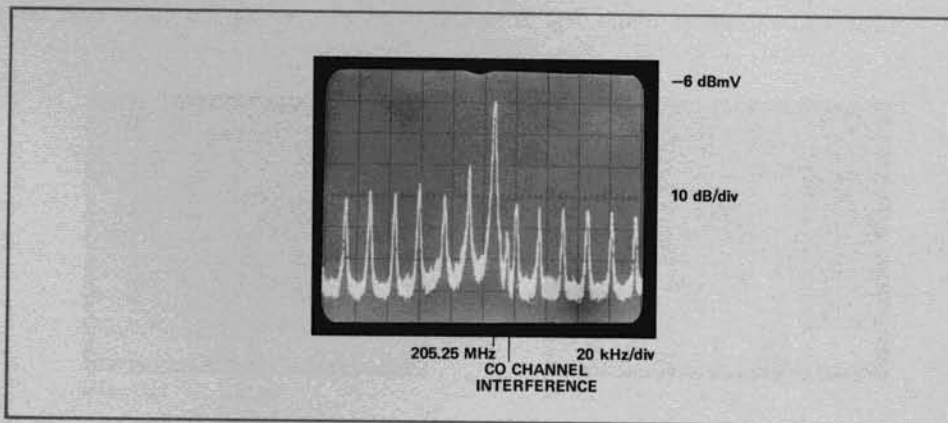
Figure 6.2 Co-channel 42 dB down at + 10 kHz Offset
